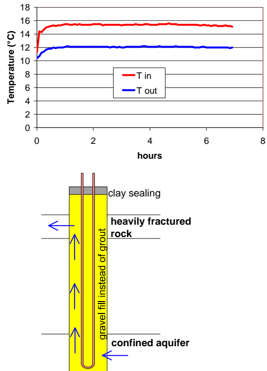
Figure 7: TRT with vertical groundwater flow along the borehole axis, temperature development (above) and explanation
